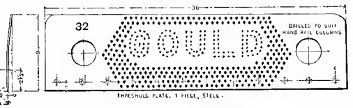
Figs. 1399-1400. Threshold-plate.
